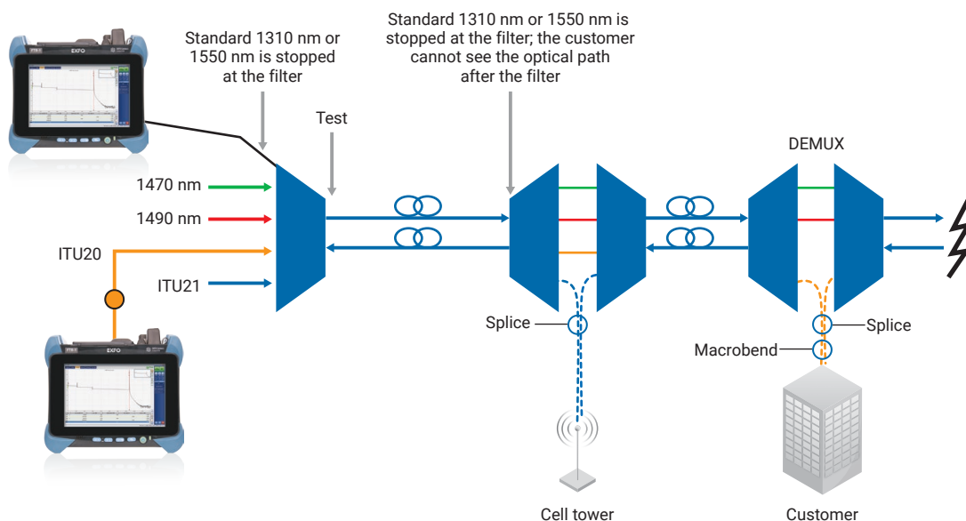
With a CWDM/DWDM OTDR, network service providers can see and validate the complete optical path prior to turning up the service.
